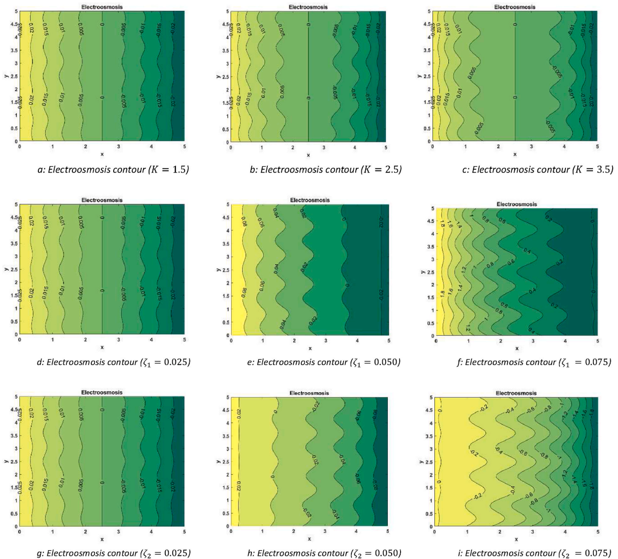
Fig. 13. Electroosmosis contours.
